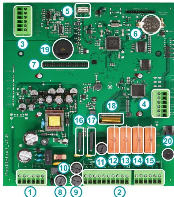
Figure: Controller board
